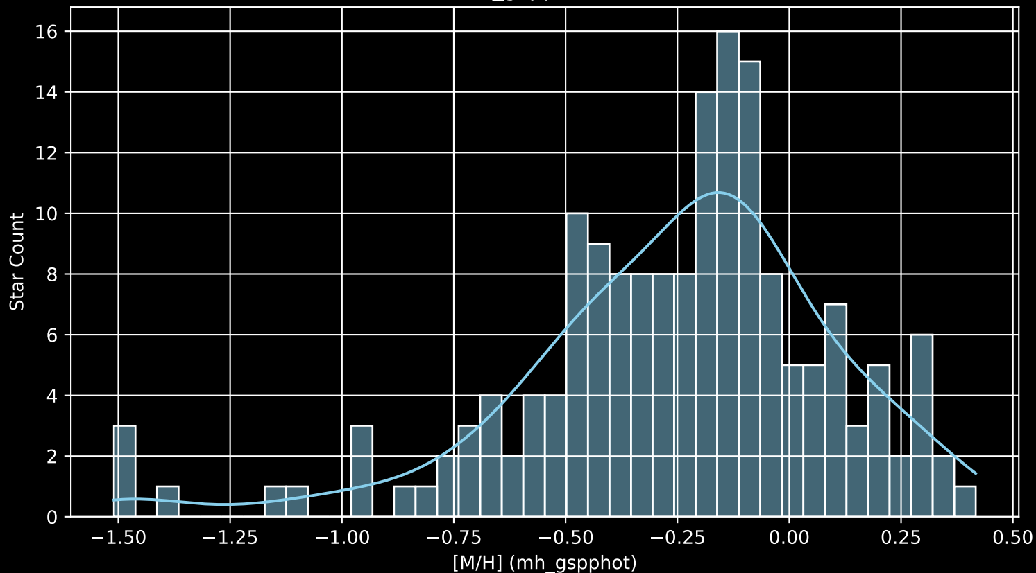
APOGEE DR17 Field: [050+63_MGA [M/H] (mh_gspphot) (n= 170)
