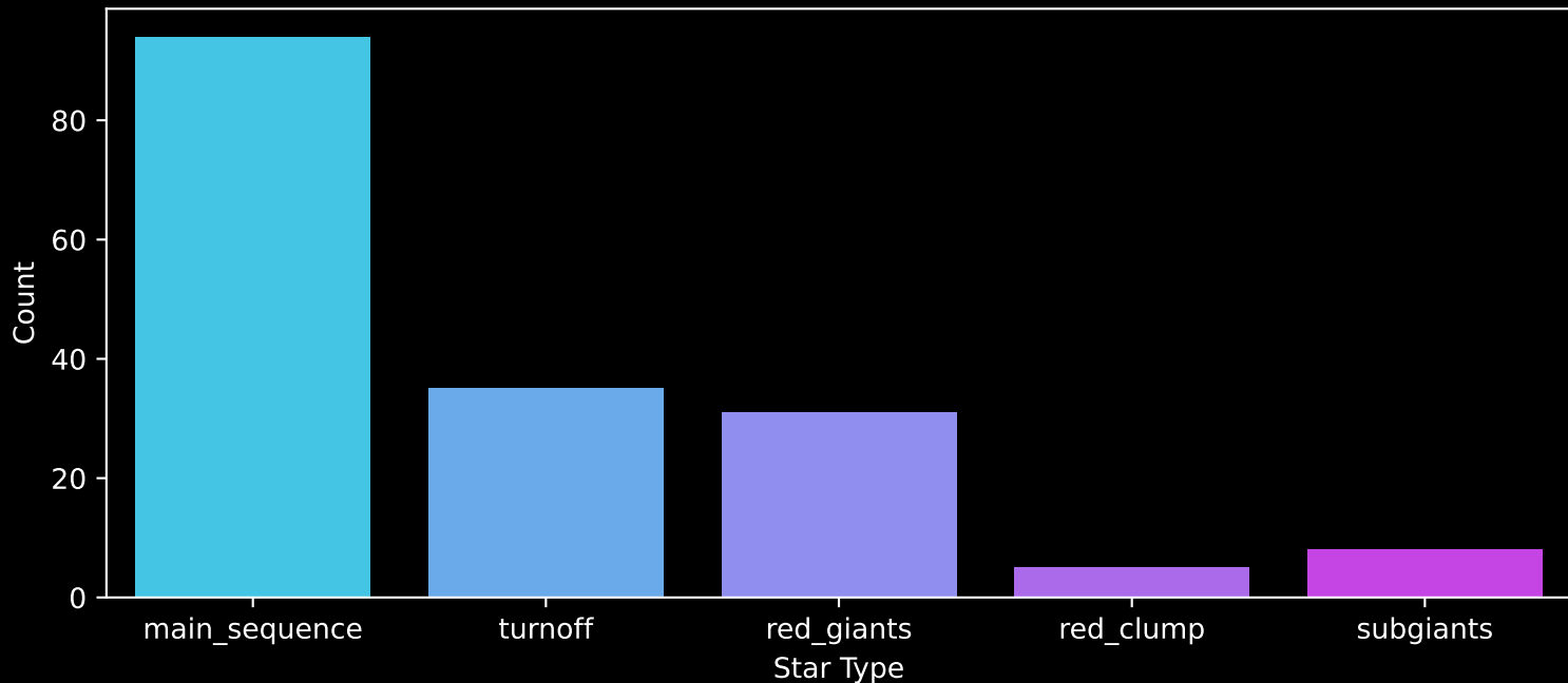
APOGEE DR17 Field: [050+63_MGA] Count plot of Star Type
