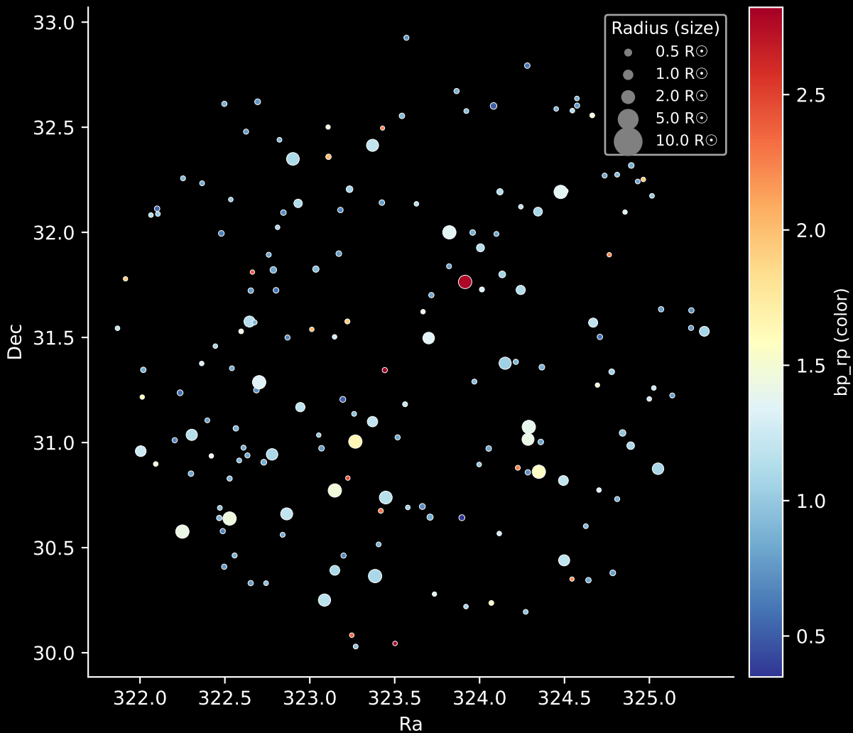
APOGEE DR17 Field: [050+63_MGA] Stars: 173
