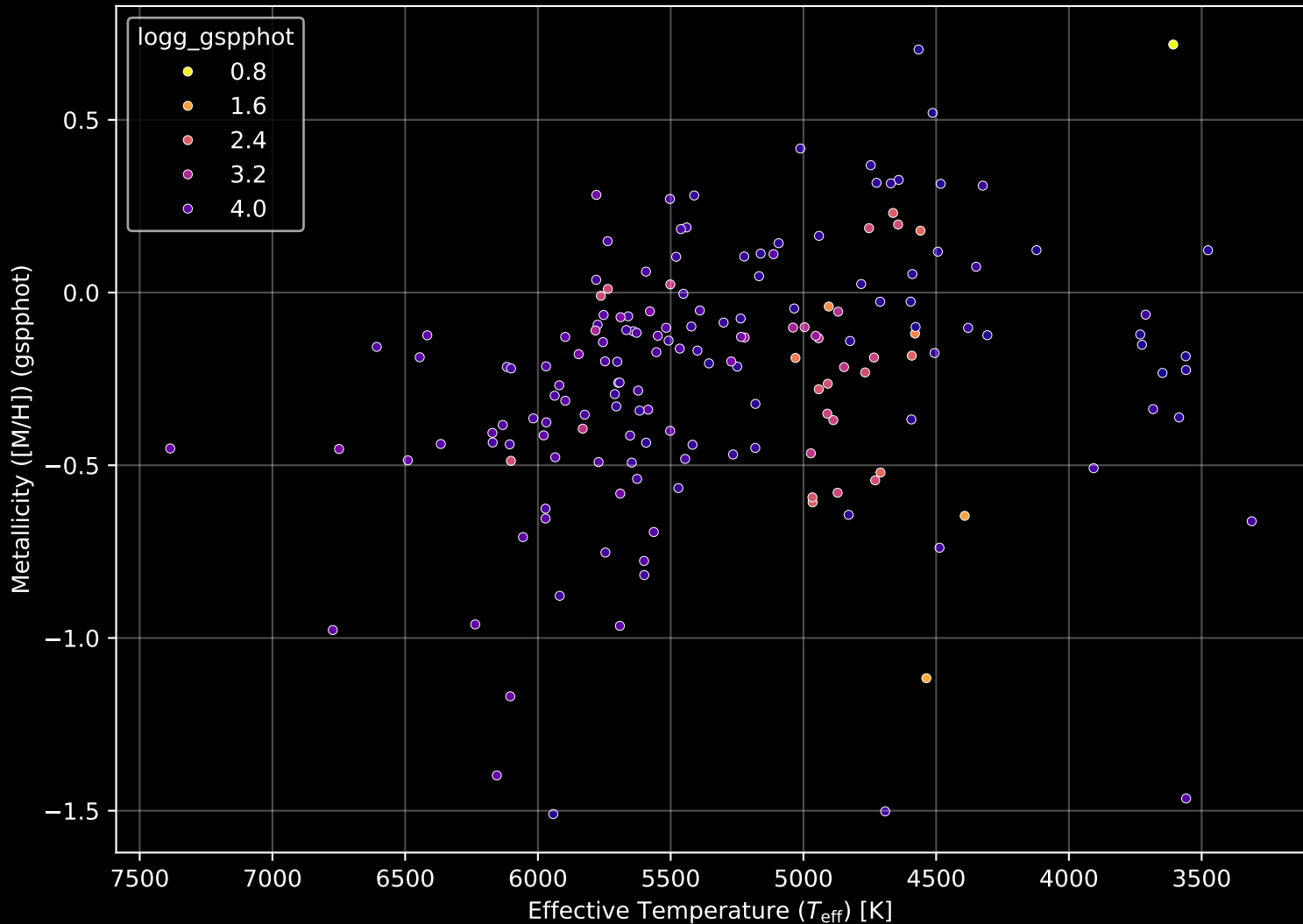
APOGEE DR17 Field: [050+63_MGA] Stellar Population Parameters (n= 173)
