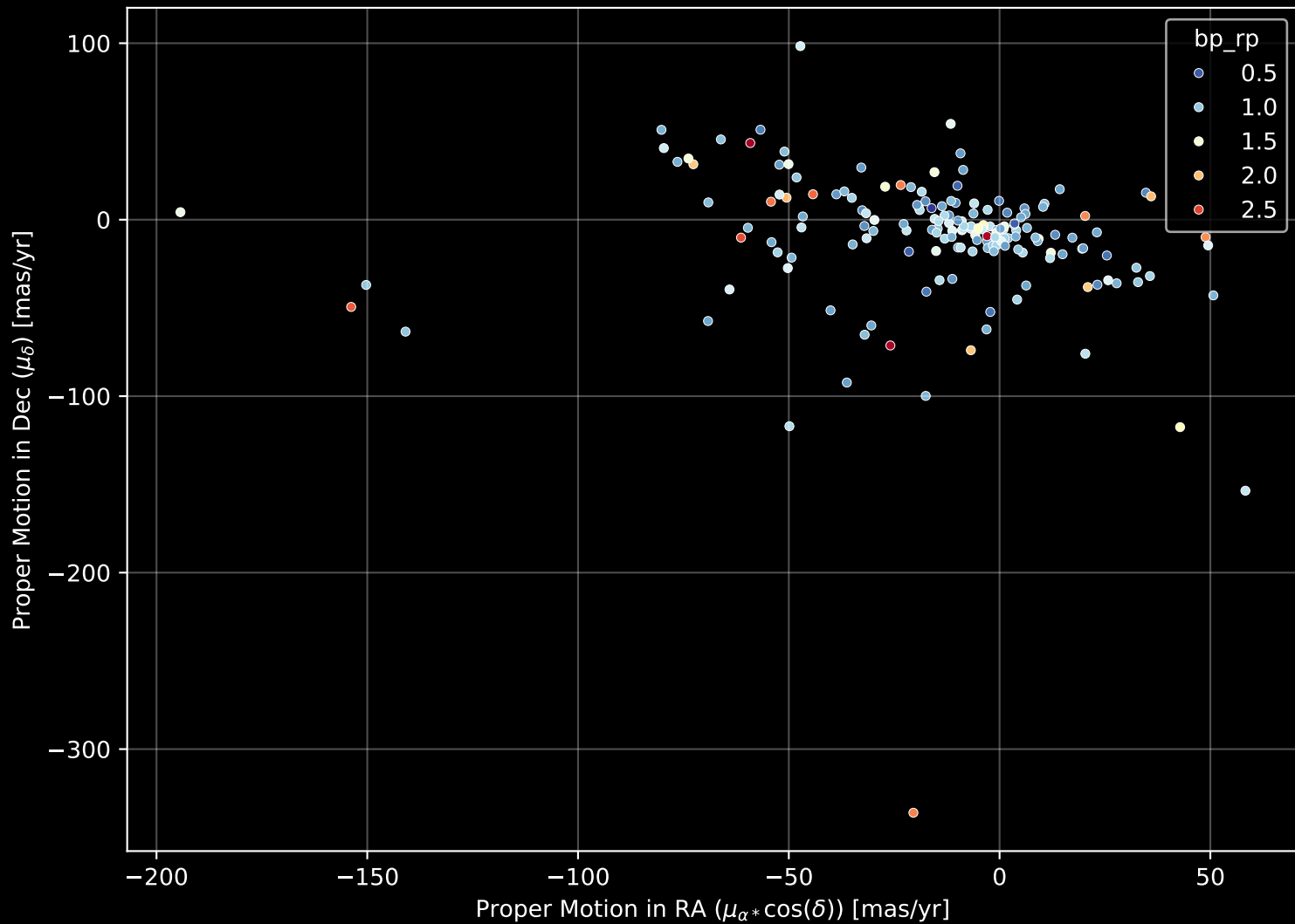
APOGEE DR17 Field: [050+63_MGA] Proper Motion Diagram (n= 173)
