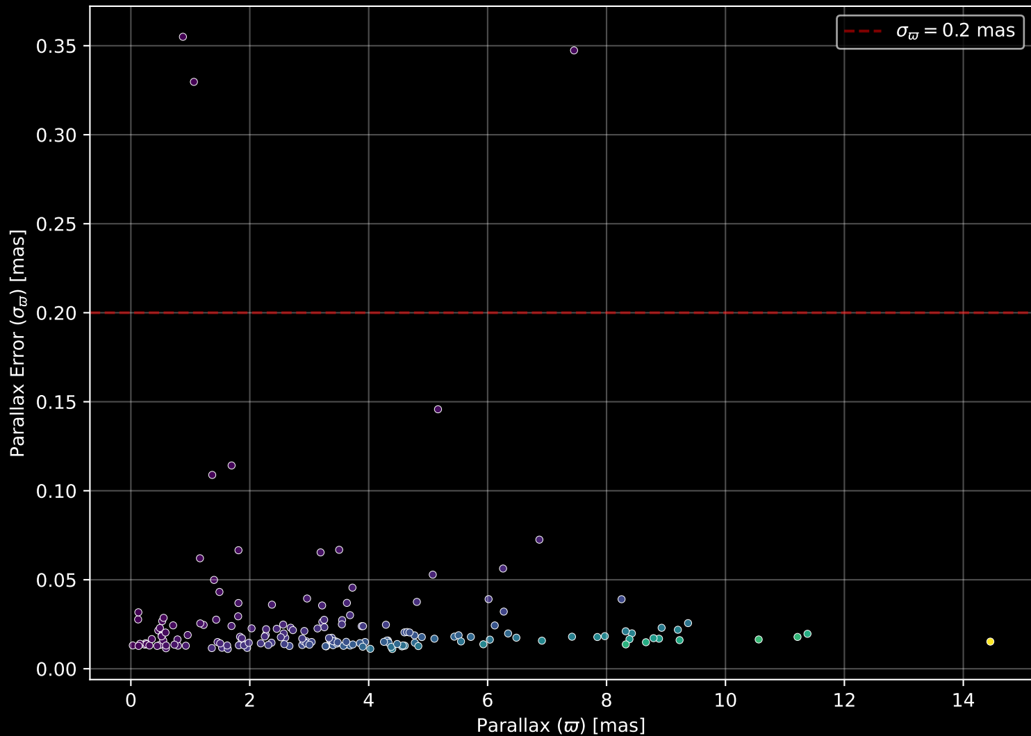
APOGEE DR17 Field: [050+63_MGA] Parallax Quality (n= 173)
