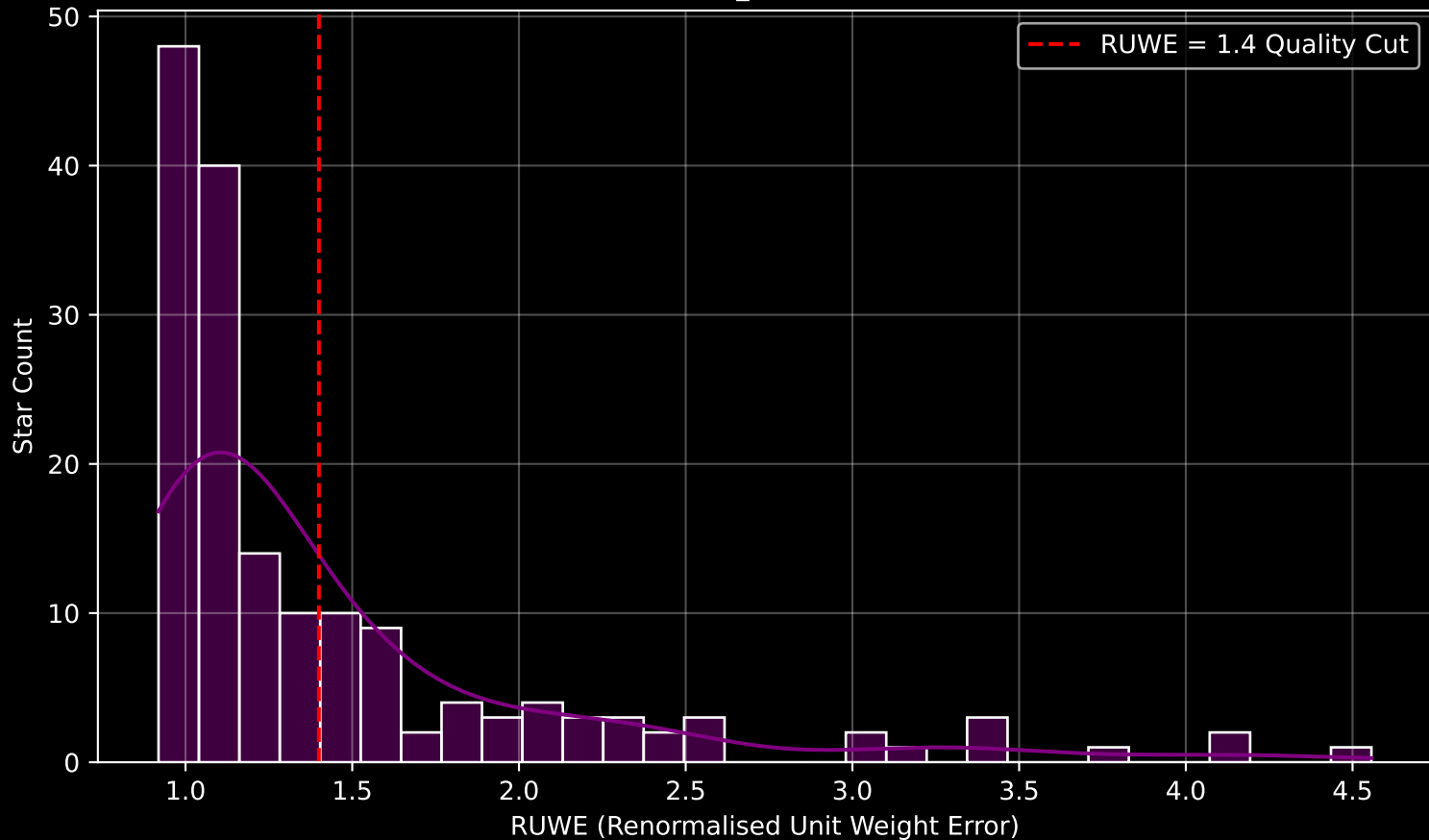
GAPOGEE DR17 Field [050+63_MGA] RUWE Distribution (n= 165)
